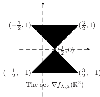
FIGURE 1. f(x_1, x_2) = \left| |x_1| + x_2 \right| + \frac{1}{2}x_1
