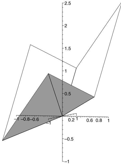
FIGURE 1. f(x_1, x_2) = \left| |x_1| + x_2 \right| + \frac{1}{2}x_1
