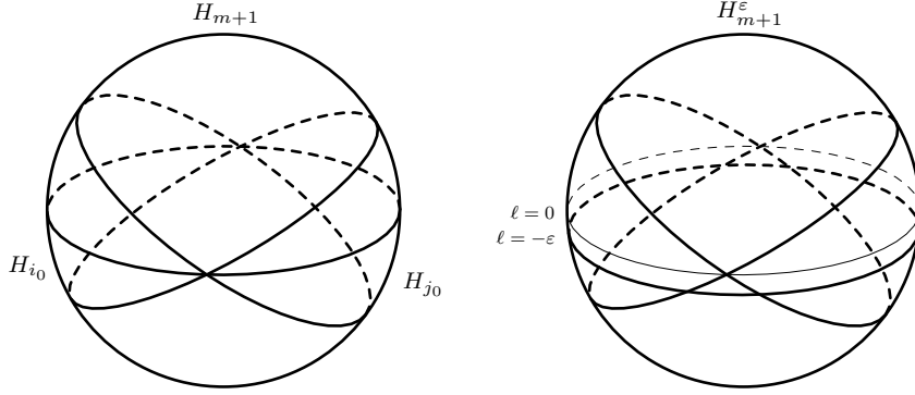
Fig. 1 Configuration for \alpha_{k_0} < \alpha_{k_0+1}
