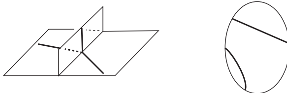
FIGURE 5. A r-embedding
