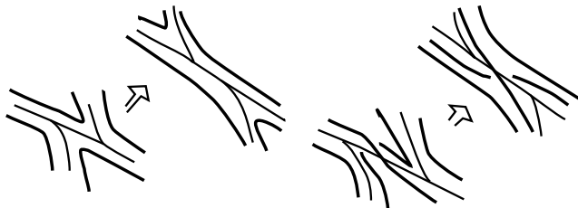
FIGURE 17. Preservation and Non-Preservation of \partial -loops
