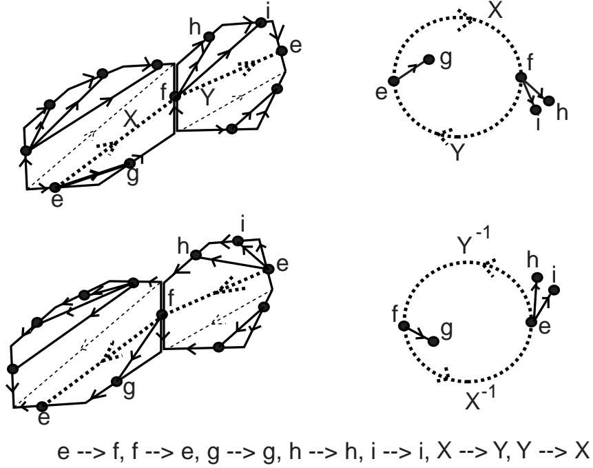
FIGURE 13. The graphs \tilde{G}_u and \tilde{G}_{-u}
