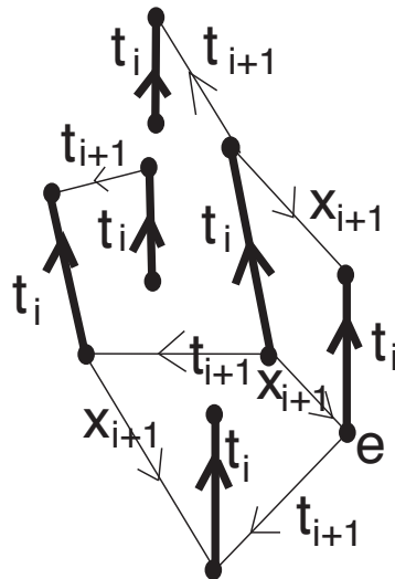
FIGURE 3. Other edges in E_i
