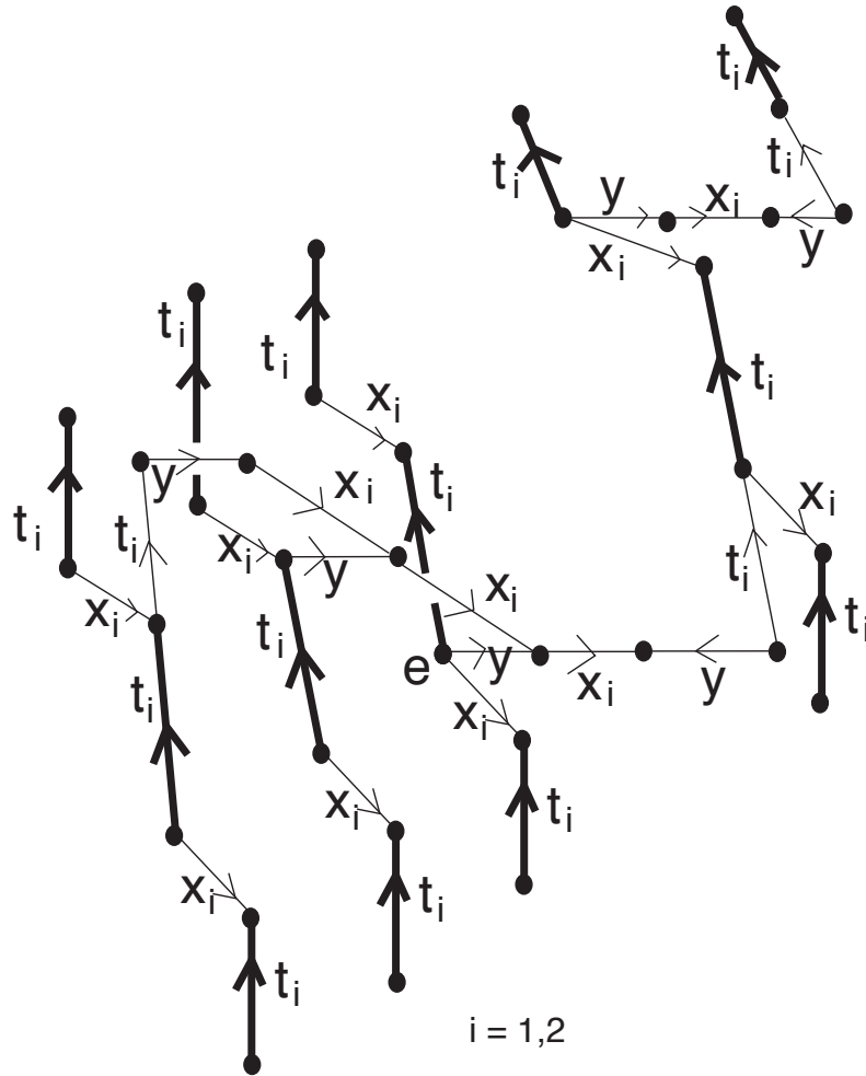
FIGURE 2. Some edges in E_i
