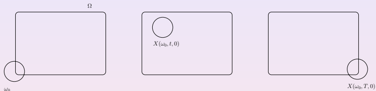
Figure: \Omega \setminus \omega(t) is not split in two disjoint connected components
